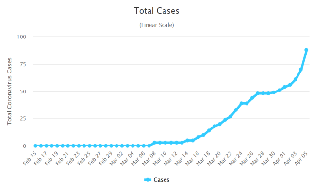
FIGURE 1. Infected cases of COVID-19 around the world [1].
