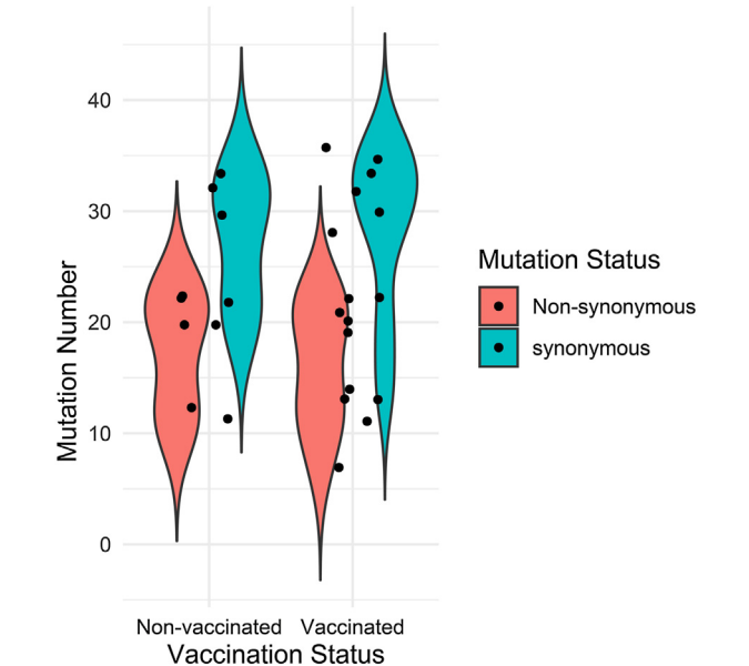
Fig. 5. Synonymous ( p=0.396 ) and non-synonymous ( p=0.083 ) mutation status between immunized and unimmunized patients.
