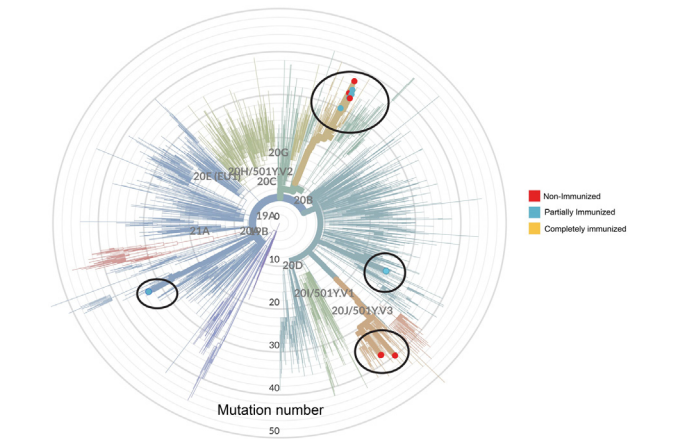
Fig. 3. Phylogenetic of tree with their existing clade with world reference genome. Red color represents unimmunized variants, sky-blue represents partially immunized and orange color represents completely immunized variants in the tree.
